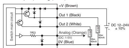
PNP Output (Analog 1-5V)
