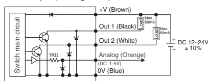
NPN Output (Analog: 1-5V)
