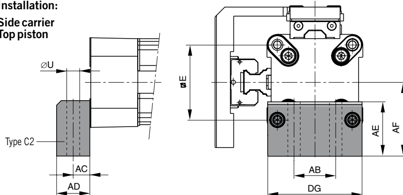
Dimension Table (mm) for End Cap Mounting Type: C1 to C4
