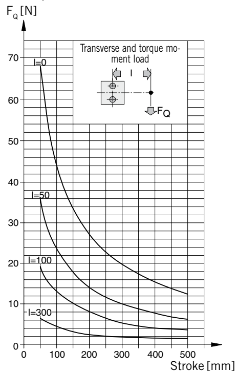
Twin Rod Cylinder 1) Transverse and Torque Moment Load - Ø 50 mm
