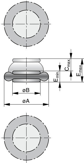
Dimension Table (mm) and Order Instructions
