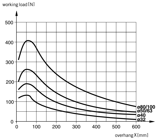
Maximum working load in relation to overhang - FEHK version with ball bearings
