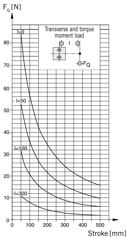
Twin Rod Cylinder 1) Transverse and Torque Moment Load - Ø 63 mm
