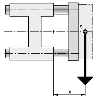
Maximum working load in relation to overhang - FEHK version with ball bearings
