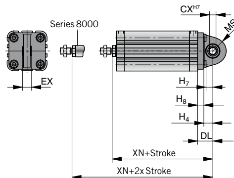
Dimension Table (mm) – Mounting BAS
