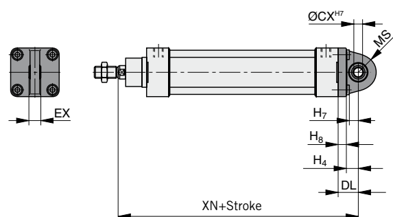
Dimension Table (mm) – for Mounting BAS
