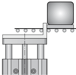
Stopping with Stop Bracket
