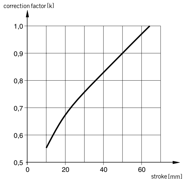
Reduction of working load with short strokes - FEHK version with ball bearings
