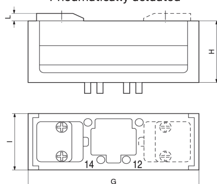
Pneumatically actuated
